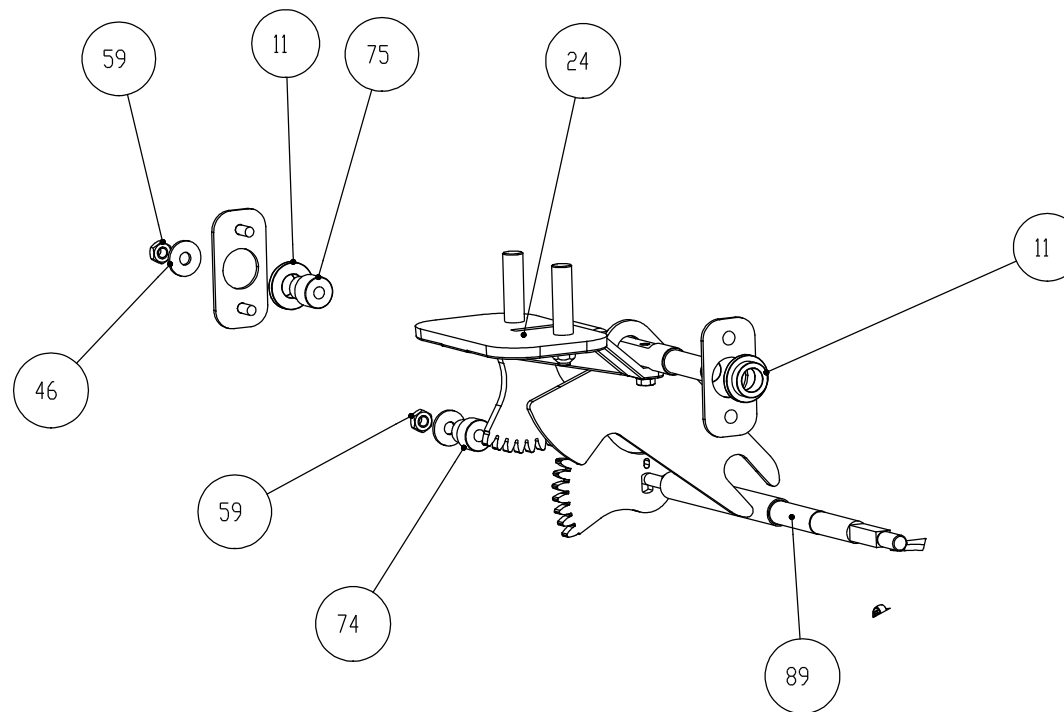
Detail B 2:5
